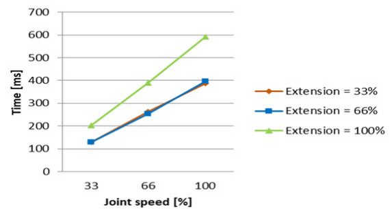
Stopping time payload 33%
