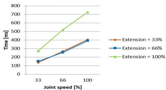
Stopping time payload 66%
