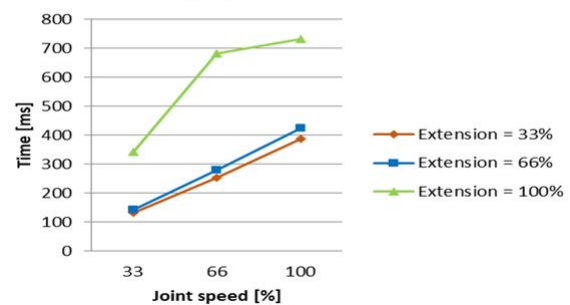
Stopping time payload 100%
