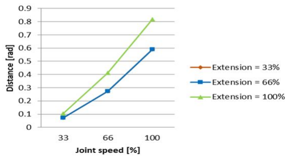
Stopping distance payload 33%
