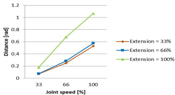
Stopping distance payload 100%
