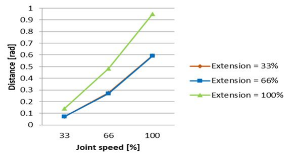
Stopping distance payload 66%
