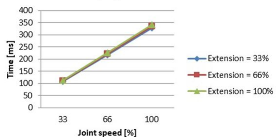
Stopping time payload 33%
