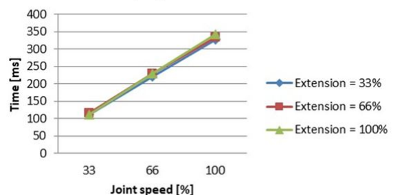
Stopping time payload 100%
